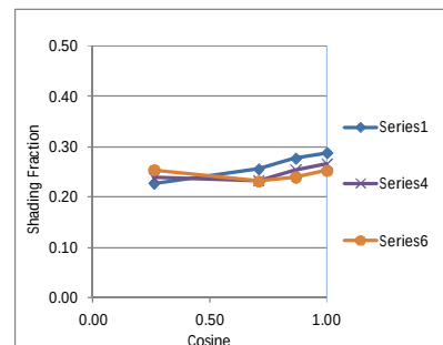
Figure B.1 Measured Solar Fractions for roller shade fabric
